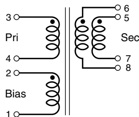
Secondary windings to be connected in parallel on PC board
