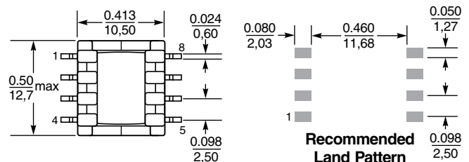
Dimensions are in inches/mm
